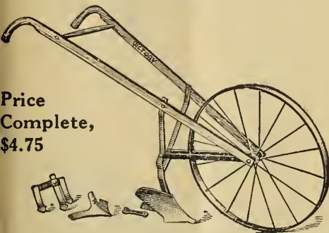
No. 600EL Horse Hoe and Cultivator
